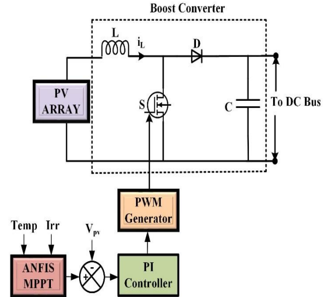
Fig.2 PV Control with ANFIS MPPT
