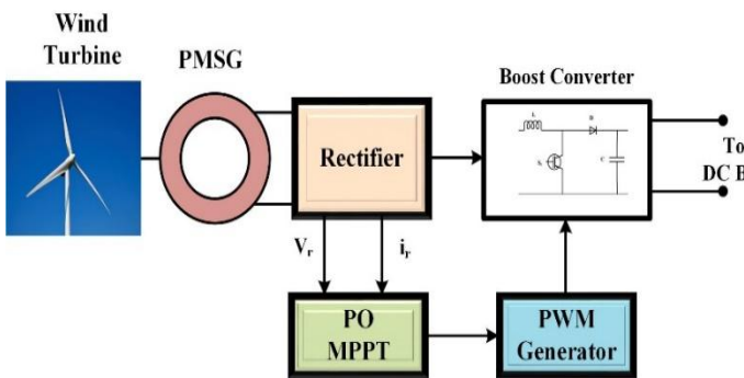
Fig.3 Wind control using PO MPPT
