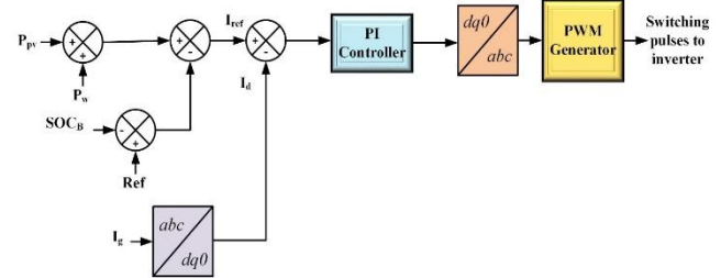
Fig.5 Inverter control using PI Controller
