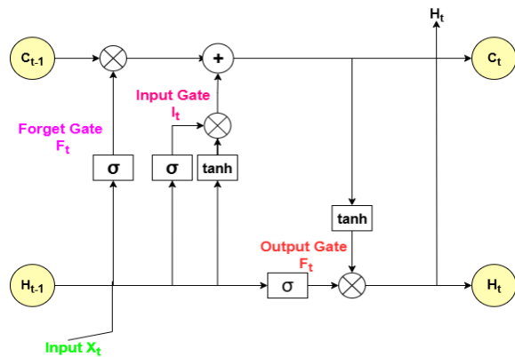
Fig.3 LSTM structure
